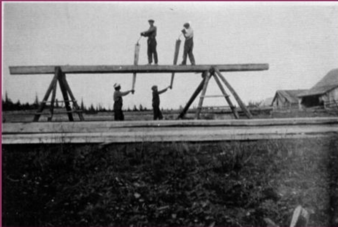
Sawing planks from a log using a whip-saw
