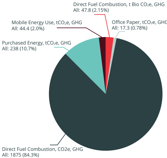
Total GHG Emissions College of New Caledonia 2025
